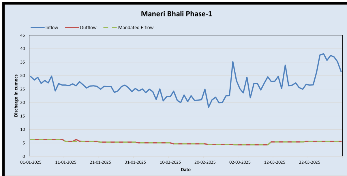
Figure 2: Graphs showing status of implementation of E-Flow at Maneri Bhali-I
