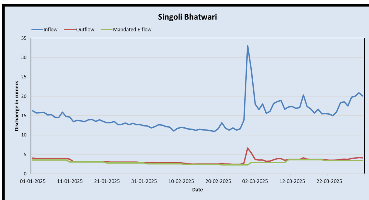
Figure 6: Graphs showing status of implementation of E-Flow at Singoli Bhatwari HEP
