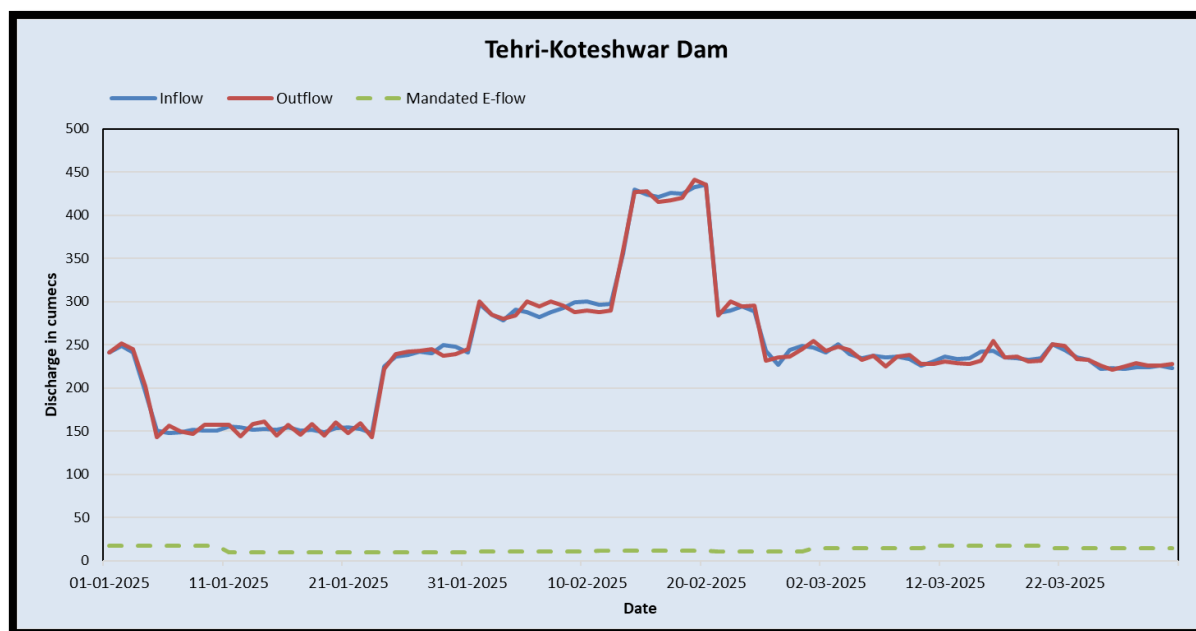
Figure 4: Graphs showing status of implementation of E-Flow at Tehri – Koteswar
